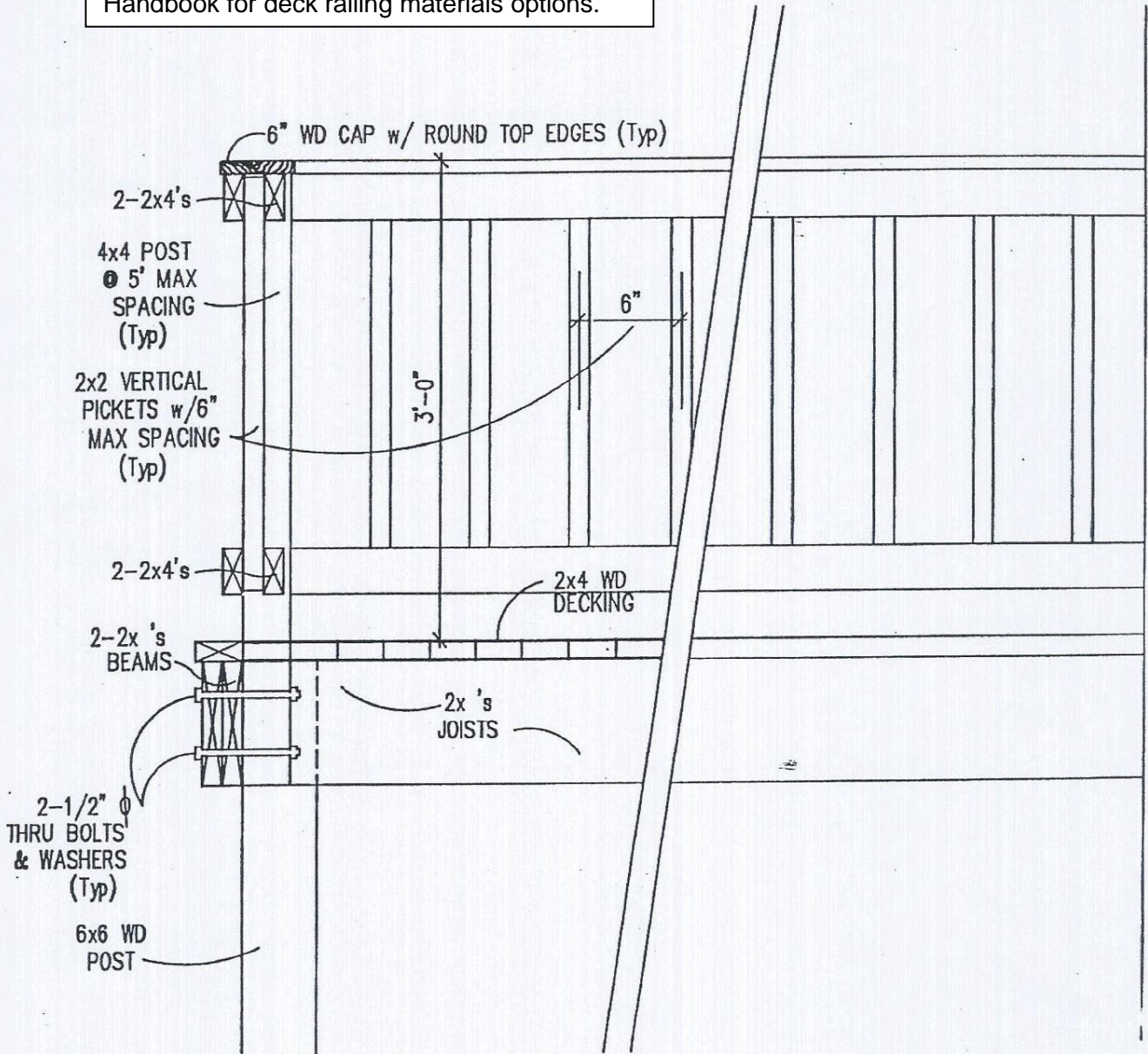
DETAIL 1
