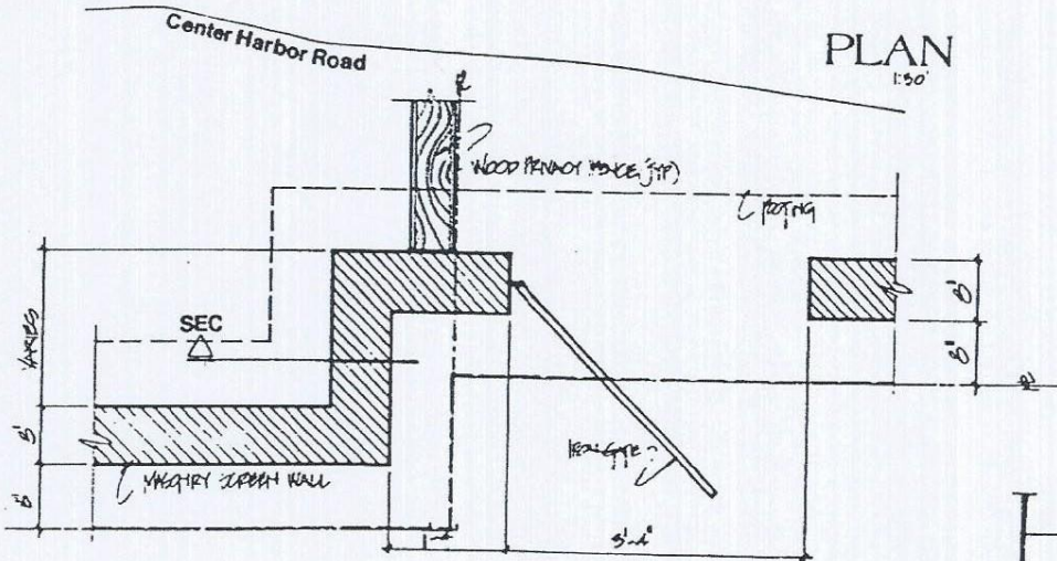
PLAN DETAIL 1/4" = 1'-0"
